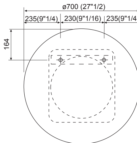
AMEM866Z
